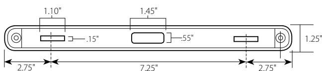
Base (front view)
