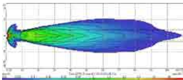
#77406 Light Output View
